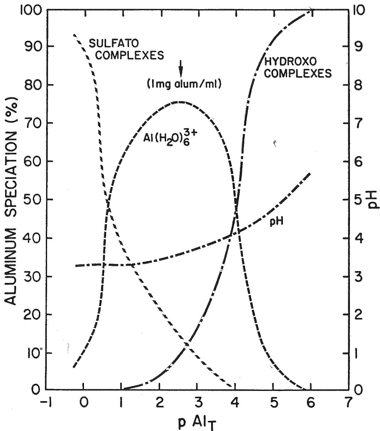
Figure 3. Calculated Speciation in Alum Stock Solutions.
