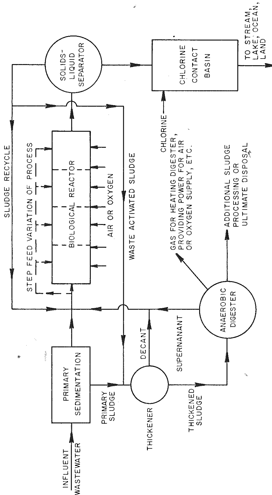
Figure 1. Simplified Flow Diagram for a Conventional Wastewater Treatment Plant.
