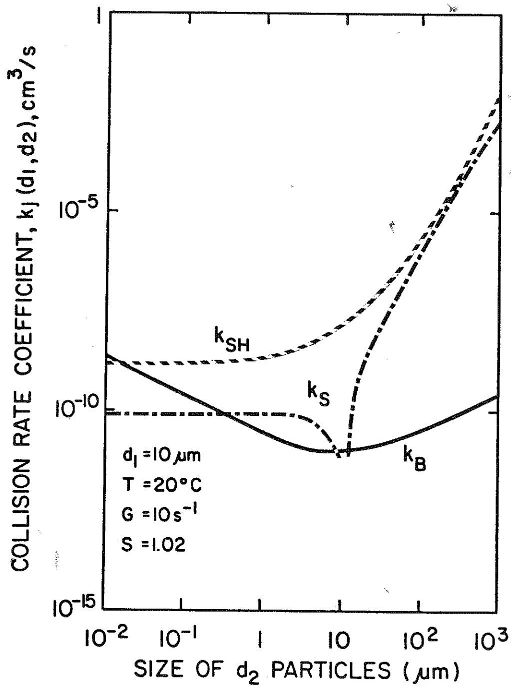
Figure 2. Comparison of Flocculation Rate Coefficients in a Flocculation Tank.
